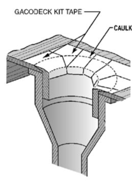
FIG. 4: Plywood Drain Detail
